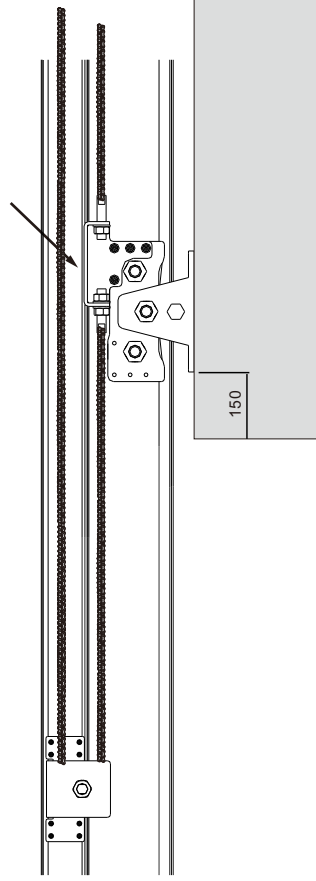
單開 Single-winged
