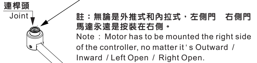
內拉式滑槽示意圖 Inward Opening Pull Arm assembly
