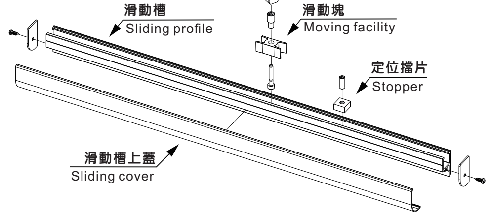
內拉式滑槽示意圖 Inward Opening Pull Arm assembly
